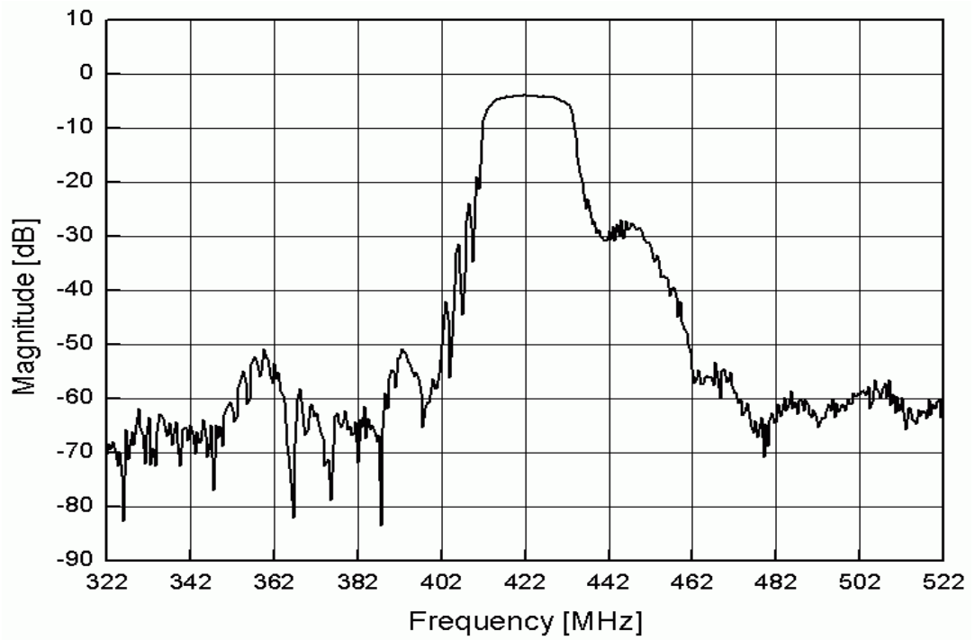
Frequency Response
